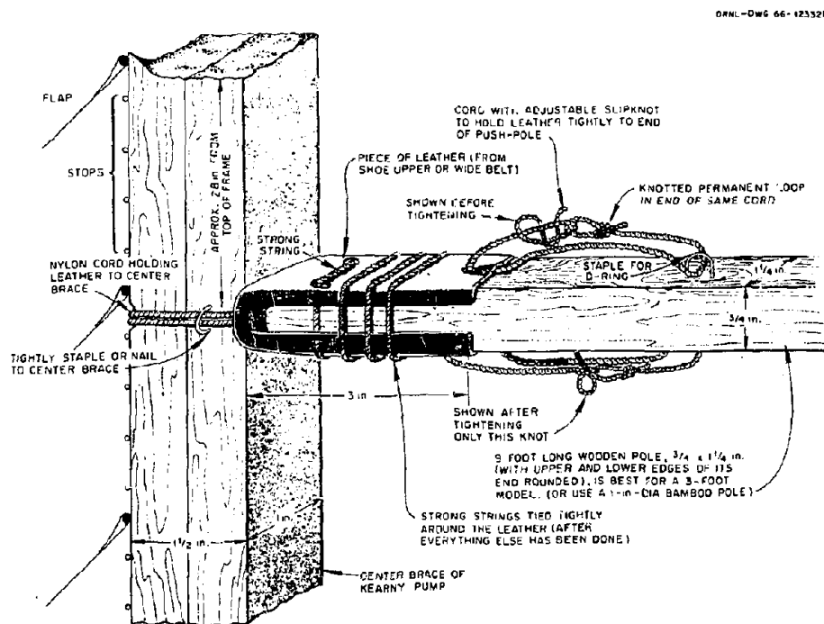
Fig. B-24. Push-pole flexible connection.
